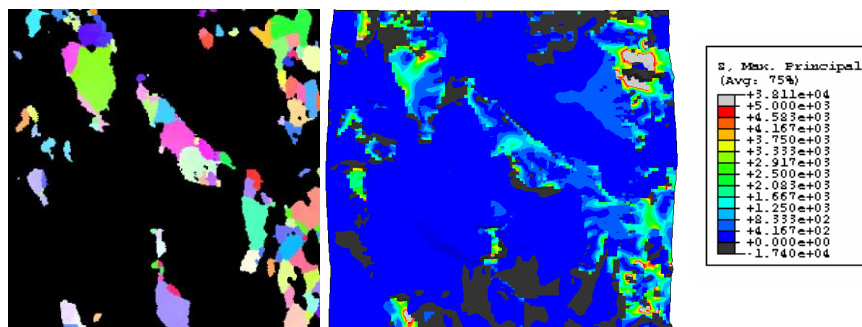
Fig.10: a) EBSD map showing carbide phase on the first layer of the aggregate. b) \sigma_{princ.max} (MPa) map on the first layer of the numerical aggregate in the composite.
