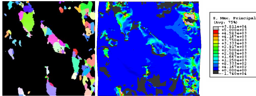
Fig.10: a) EBSD map showing carbide phase on the first layer of the aggregate. b) \sigma_{\text{princ.max}} (MPa) map on the first layer of the numerical aggregate in the composite.
