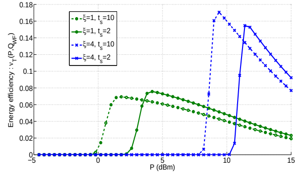
Fig. 1. Energy efficiency ( \nu_T ) in bits/J v.s transmit power ( P ) in dBm for a MIMO system with imperfect CSITR, M = N = 2 , R_0 = 1\text{bps} , T_s = 100 , \frac{b}{a} = 10\text{ mW} for certain values of \xi and t_s .
