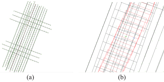
Fig. 2. Flight plan for the 2004 aerial-image acquisition campaign for the city of Marseille. (a) Total of 23 flight-strips are flown, six of which are perpendicular. Dots on each flight strip: the position where an image is captured. (b) Enlarged detail of flight strips 19–21 illustrating the 60% overlap between images taken on the same strip and 60% between two adjacent strips. Areas covered by images taken in each strip is presented by a bounding rectangle.
