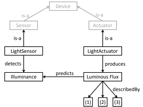
Figure 7. Specialization of the abstract ontology level to account for a specific effect: the emission of light. (1), (2) and (3) refer to the corresponding formulae defined in the text.
