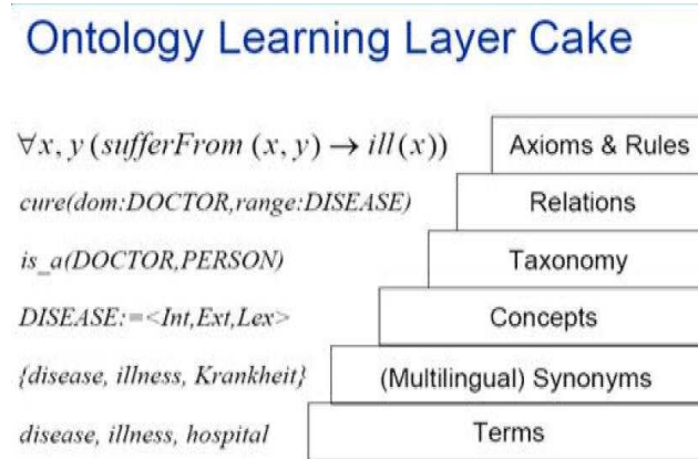
Fig. 1.8. Ontology Learning Process [56]
