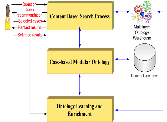
Figure1. Multi-Domain Content-Based Search based on case-based modular ontology and Ontology learning.
