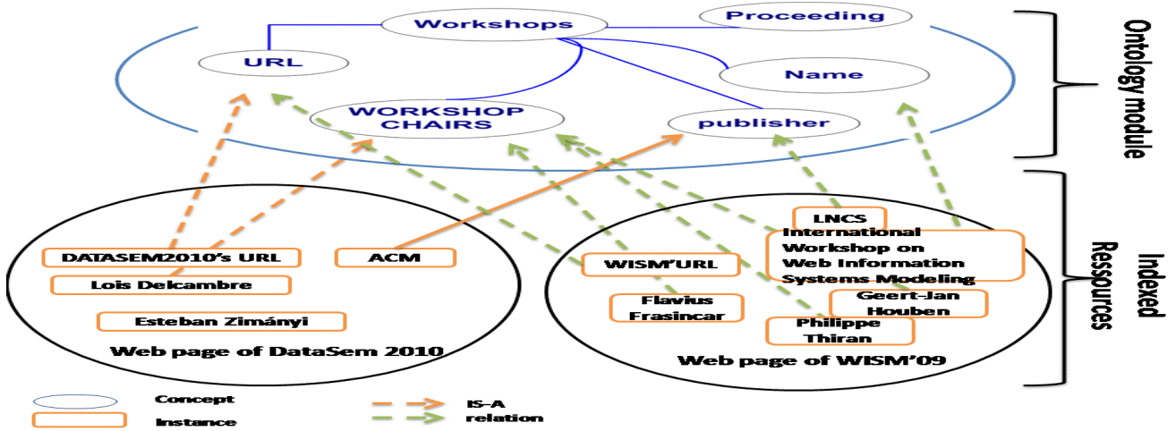
Figure 3. Relation between resources and the second layer
