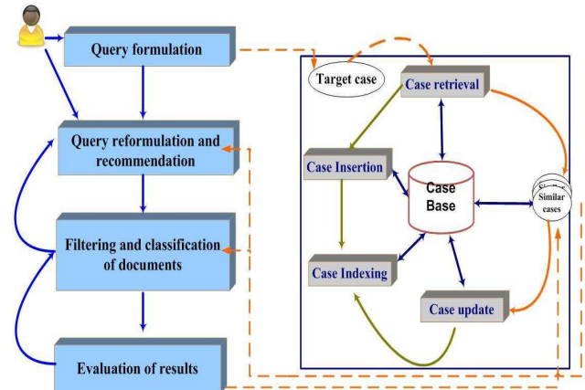
Figure 4. CBR mechanism for semantic search
