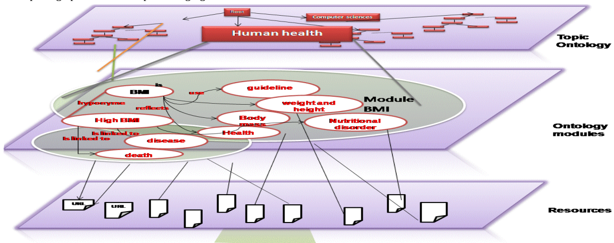
Figure 2. Multi-layer ontology warehouse for semantic search
