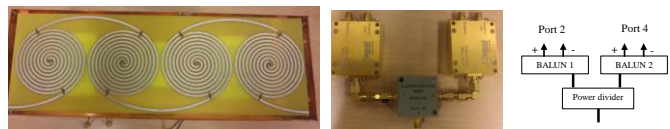
Fig. 5. The antenna array and the used feeding circuit composed of two pulse lab PSPL BALUN and a power divider in the middle of the photography.
