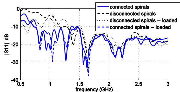
Fig. 7. The reflection coefficient presented as a function of the frequency for the different configurations described in Fig. 6.
