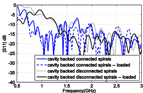
Fig. 10 The reflection coefficient presented as a function of the frequency for the different cavity backed antenna configurations (Fig. 6).
