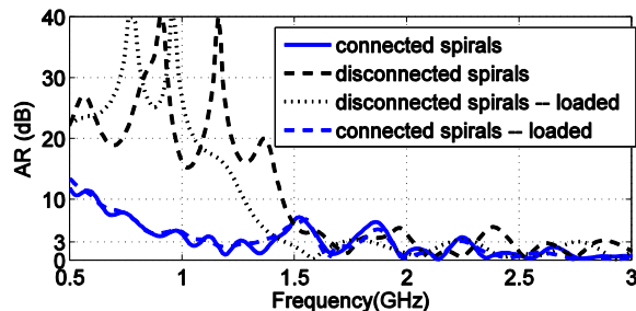
Fig. 8. The Axial Ratio presented as a function of the frequency for the different antenna configurations (Fig. 6).
