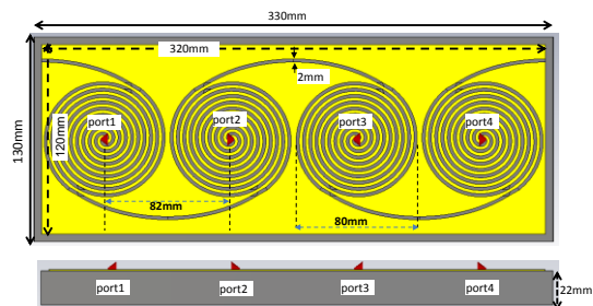
Fig. 4. (up) The antenna array considered for our investigations. The microstrip line width is 2mm, the distance between spirals is 82mm and the FR4 substrate thickness is 0.8mm. (down) The cavity is placed at 22mm from the bottom of the array.
