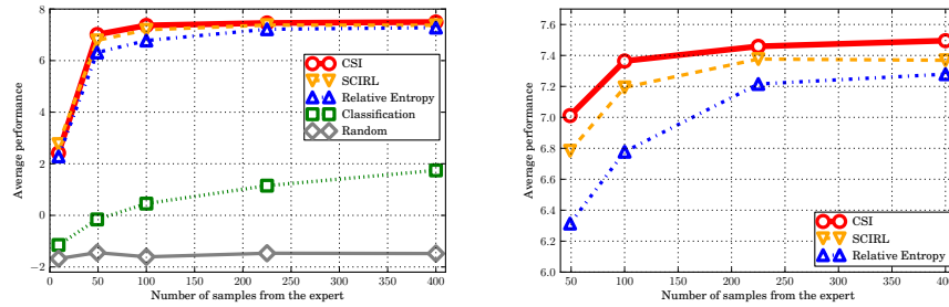
(a) Mean performance over 100 runs on the (b) Zoom of Fig 2a showing the ranking of Highway driving problem. the three IRL algorithms.
