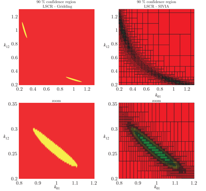
Fig. 2. Gridding (left) and paving (right) of search space obtained using LSCR in the two-compartment model case for the characterization of the confidence region \Theta_{r,q}^\varepsilon ; the two bottom subfigures are obtained by zooming in on one of the connected components of \Theta_{r,q}^\varepsilon
