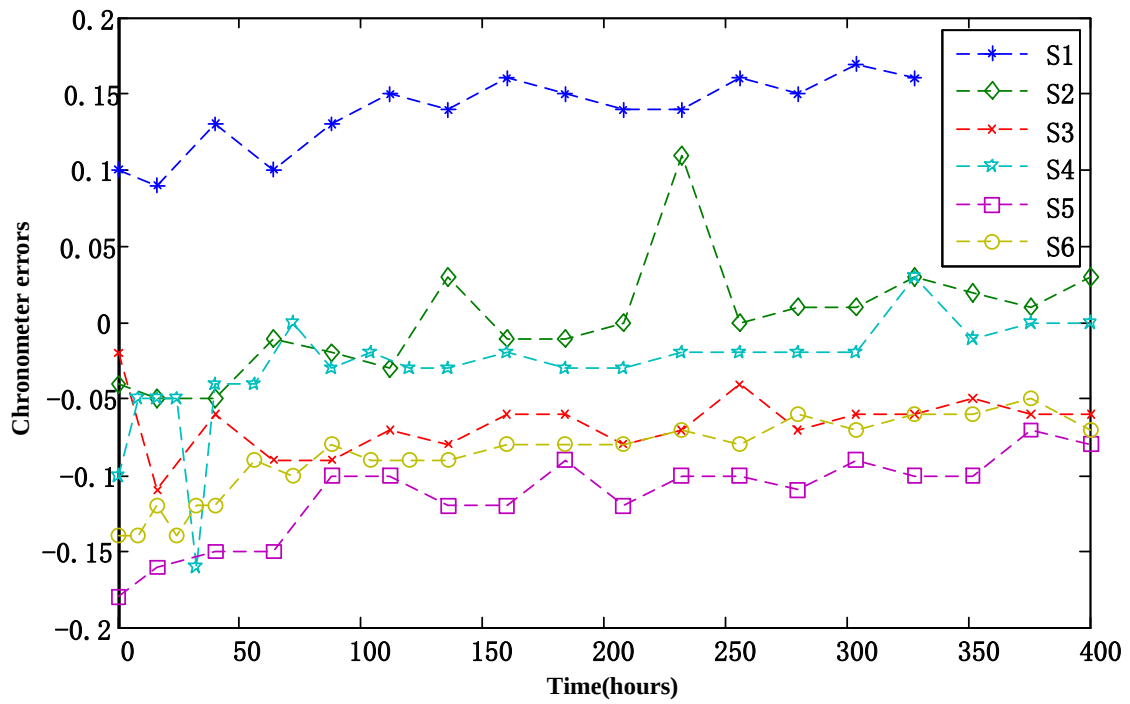
Figure 8. Degradation path of CE of sample No. 5000101 under different designs
