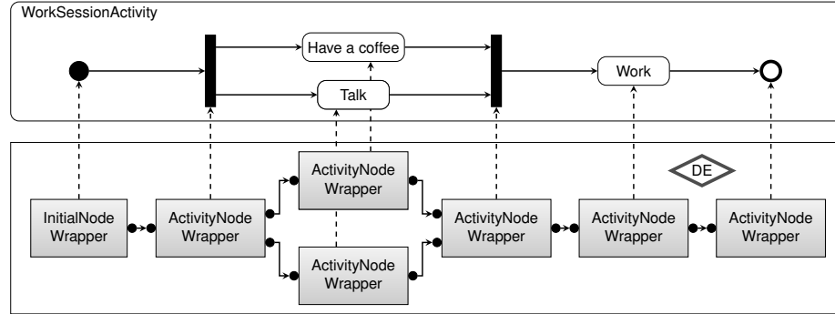
Fig. 9. Example fUML model and its wrapping ModHel’X model using DE.
