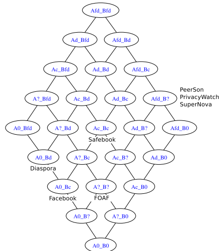
Figure 1. Lattice based on the Data Encryption (A) and Traffic Communication Encryption (B) properties.
