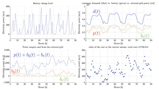
Figure 8. Powe usage.
