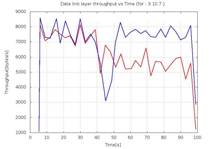
Fig. 10. MAC throughput at node 21 from node 24.
