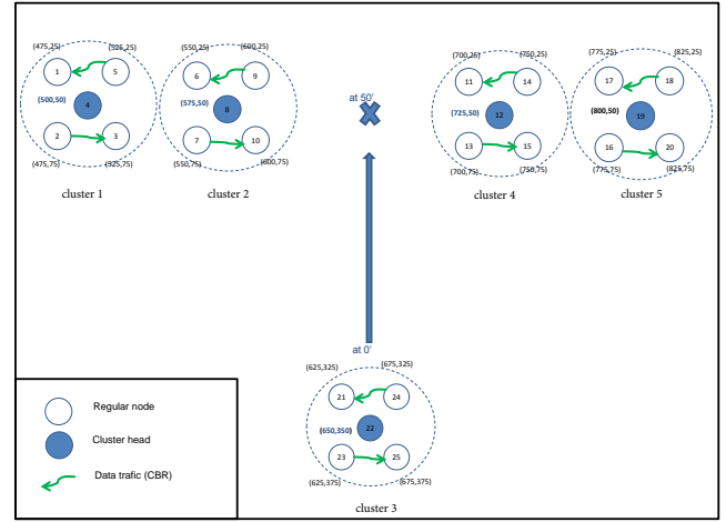
Fig. 5. Scenario description used in the CORASMA simulator (distances in meter).
