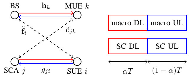
Fig. 2. A two-tier network employing TDD protocol; solid arrows denote direct links and dashed arrows denote interfering links.
