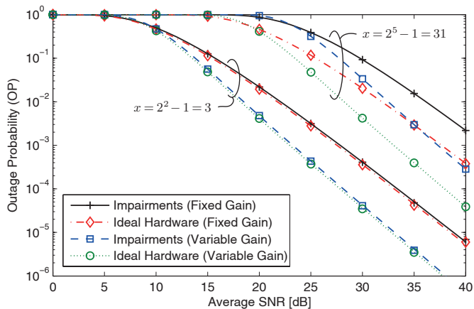
Fig. 2. Outage probability P_{\text{out}}(x) for AF relaying with ideal hardware and with hardware impairments of \kappa_1 = \kappa_2 = 0.1 .
