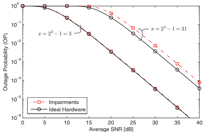
Fig. 3. Outage probability P_{\text{out}}(x) for DF relaying with ideal hardware and with hardware impairments of \kappa_1 = \kappa_2 = 0.1 .
