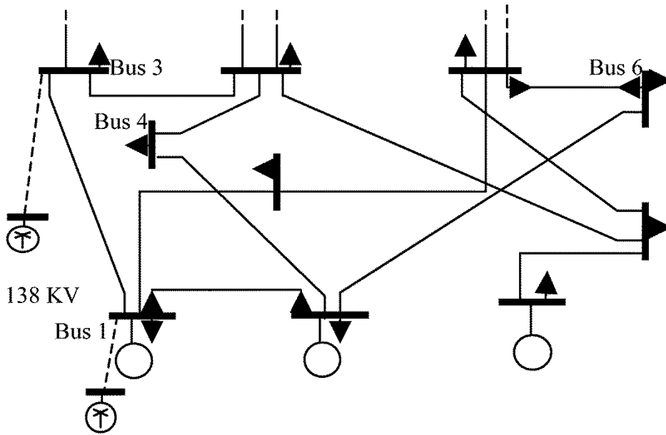
Figure 8. The two 300 MW WECS at Buses 1 and 3 in the MRTS [31].
