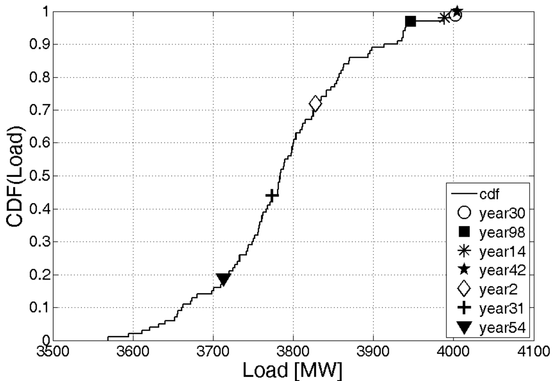
Figure 15 Cumulative distribution function of load demand at hour 8443.
