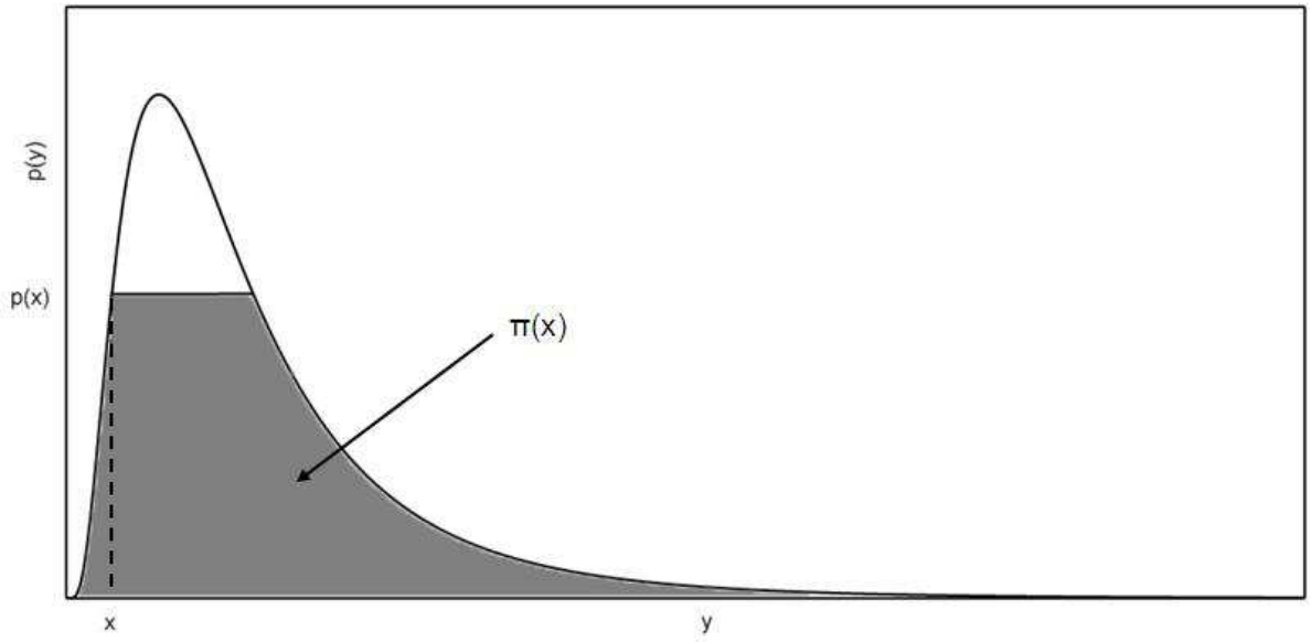
Figure 6 Transformation (iii); the value of the possibility function \pi^f at x equals the shaded area.
