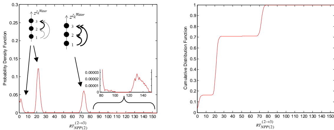
Figure 20: Probability density function (PDF) (on the left) and respective cumulative distribution function (CDF) (on the right) of the time ( RT ) necessary to restore the healthy state (3) of the nuclear power plant (NPP), given that it entered in a marginal state (2) after the earthquake occurrence.
