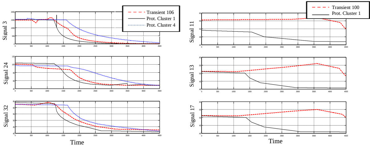
Figure 6; Left: evolution of signals 3, 24 and 32 in transient 106 and in the prototypical transients of clusters 1 and 4. Right: evolution of signals 11, 13 and 17 in transient 100 and in the prototypical transient of cluster 1
