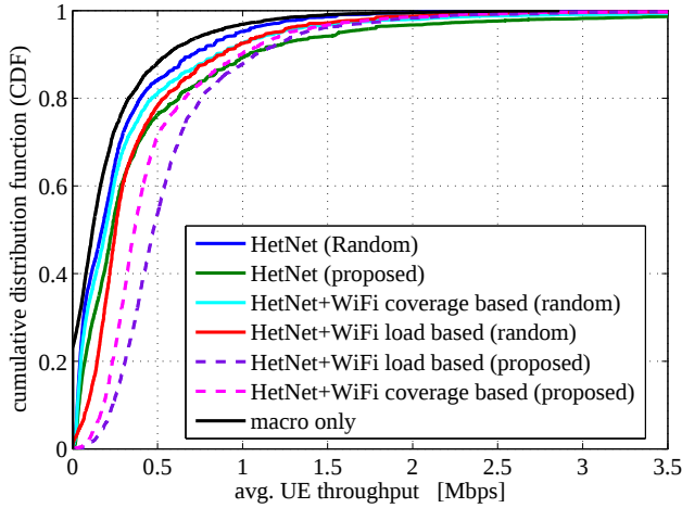
Fig. 4. Cumulative distribution function (CDF) of the average UE throughput for N_{UE} = 30 UEs and K = 2 SCBSs per macrocell sector.
