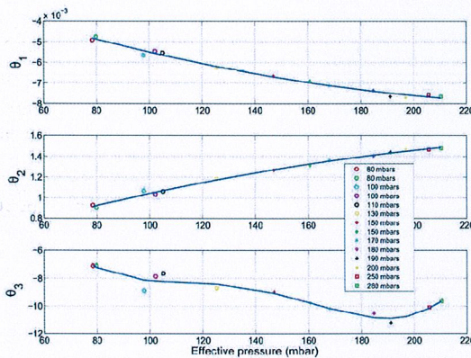
Fig. 8. Evolution of the local parameters models with respect to the pressure p (markers) and the polynomial models (2) (solid line)
