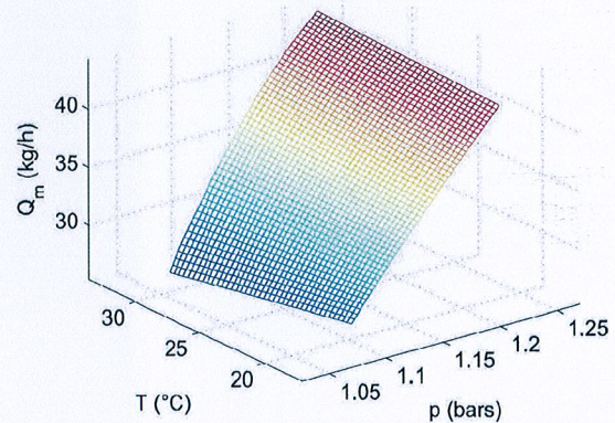
Fig. 14. Simulation of the Q_m estimated model defined by (4) for a fixed control signal at 50 %
