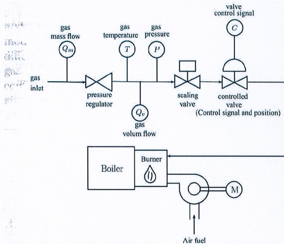
Fig. 1. Schematic view of the boiler
