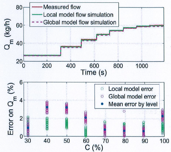
Fig. 10. Local model and one scheduling input global model simulations with 200 mbar experiment data
