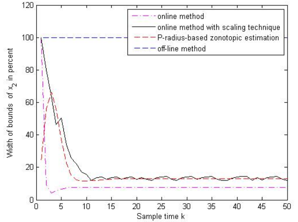
Fig. 5. Comparison of the bound's width of x_2
