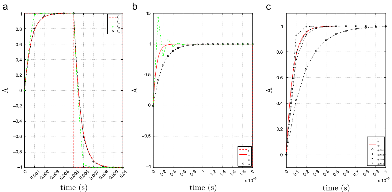
Fig. 3. q -Axis current response for different tunings of the current closed-loop. (a) T_e = 1 ms, r_1 = 0.65 , r_2 = 0.65 , N = 1 , (b) T_e = 100 \mu s, r_1 = 19.5 , r_2 = 19.5 , N = 1 , (c) T_e = 100 \mu s, r_1 = 19.5 , r_2 = 19.5 , N = 1 to 4.
