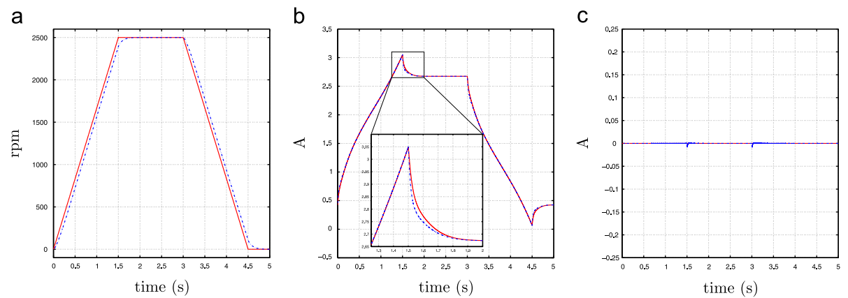
Fig. 6. Simulation of the sampled-data IDA-PBC with a sampled period equal to 200 \mu\text{s} . (a) \Omega^*(-), \Omega(-) , (b) i_q^*(-), i_q(-) , (c) i_d^*(-), i_d(-) .
