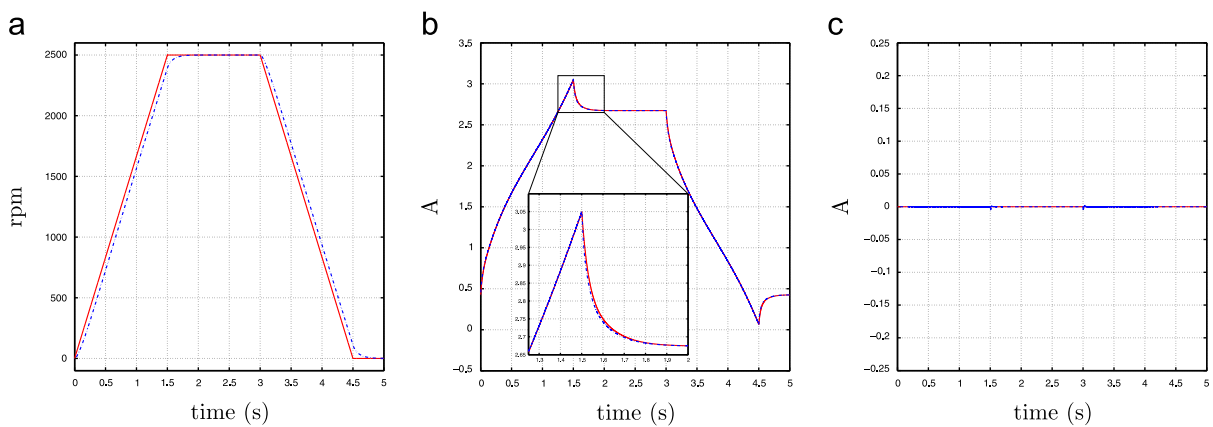
Fig. 7. Simulation of the sampled-data IDA-PBC with a sampled period equal to 500 \mu\text{s} . (a) \Omega^*(-), \Omega(-) , (b) i_q^*(-), i_q(-) , (c) i_d^*(-), i_d(-) .
