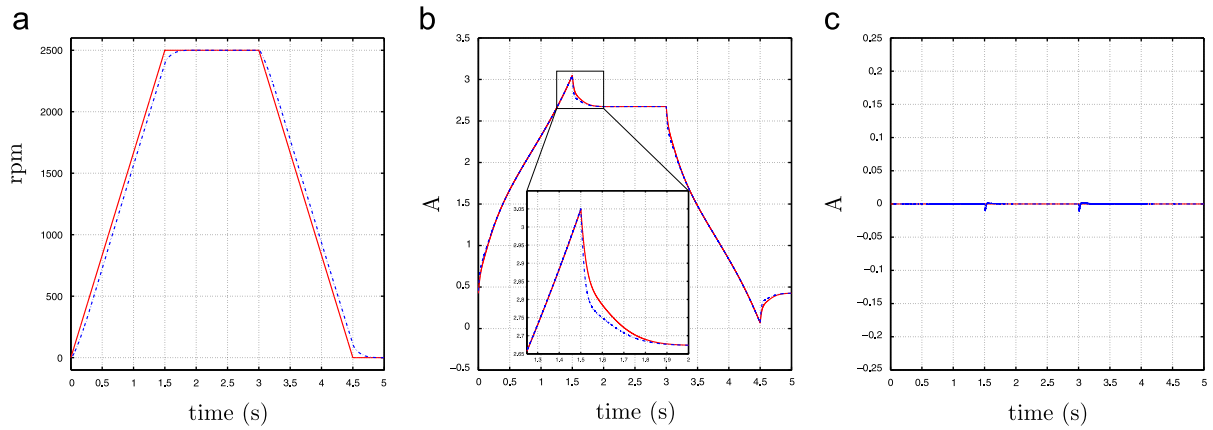
Fig. 5. Simulation of the emulated IDA-PBC with a sampled period equal to 200 \mu\text{s} . (a) \Omega^*(-), \Omega(-) , (b) i_q^*(-), i_q(-) , (c) i_d^*(-), i_d(-) .
