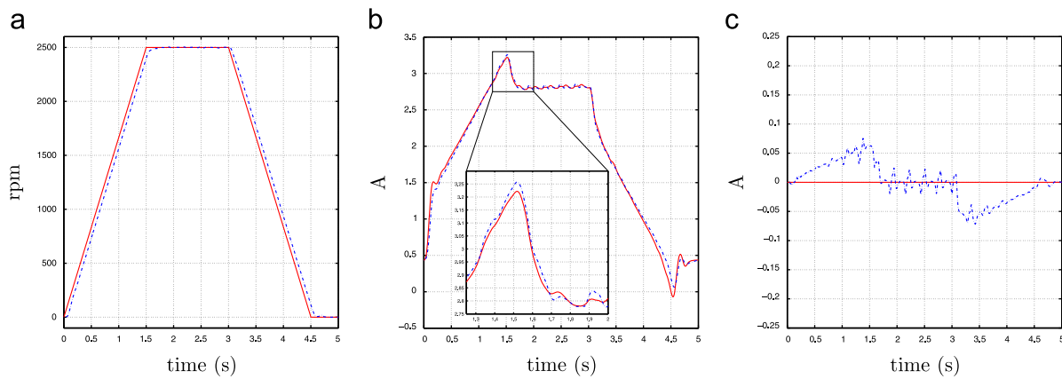
Fig. 9. Experimentation of the sampled-data IDA-PBC with a sampled period equal to 500 \mu s. (a) \Omega^*(-) , \Omega(-) , (b) i_q^*(-) , i_q(-) , (c) i_d^*(-) , i_d(-) .
