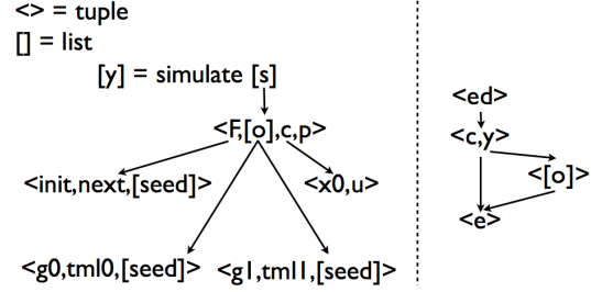
Figure 1: Simulation syntax tree.
