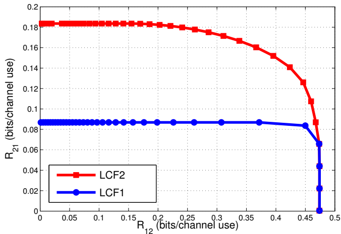
(b) P_1 = 10 dB, P_2 = P_R = 5 dB, |h_1|^2 = 6 , |h_2|^2 = 0.5
