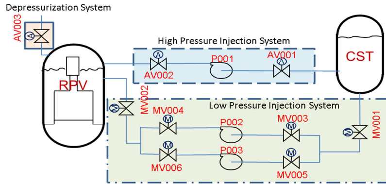
Figure 5-1: Simplified NPP layout
