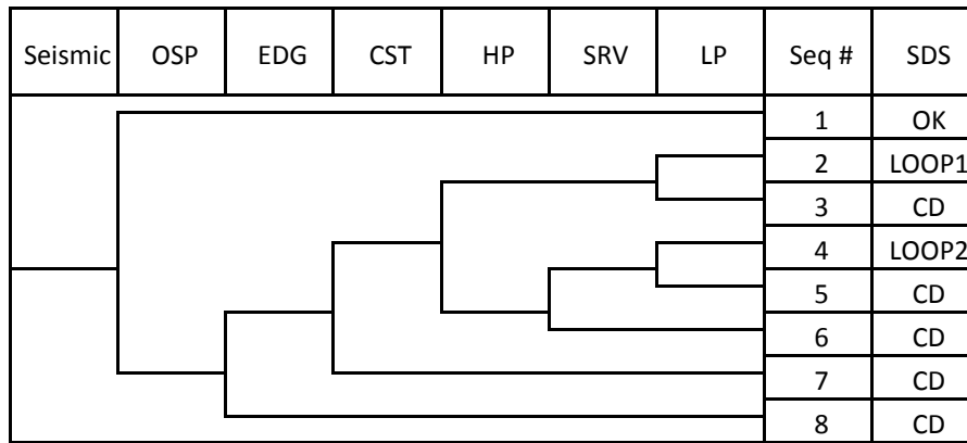
Figure 5-3: Seismic Event Tree
