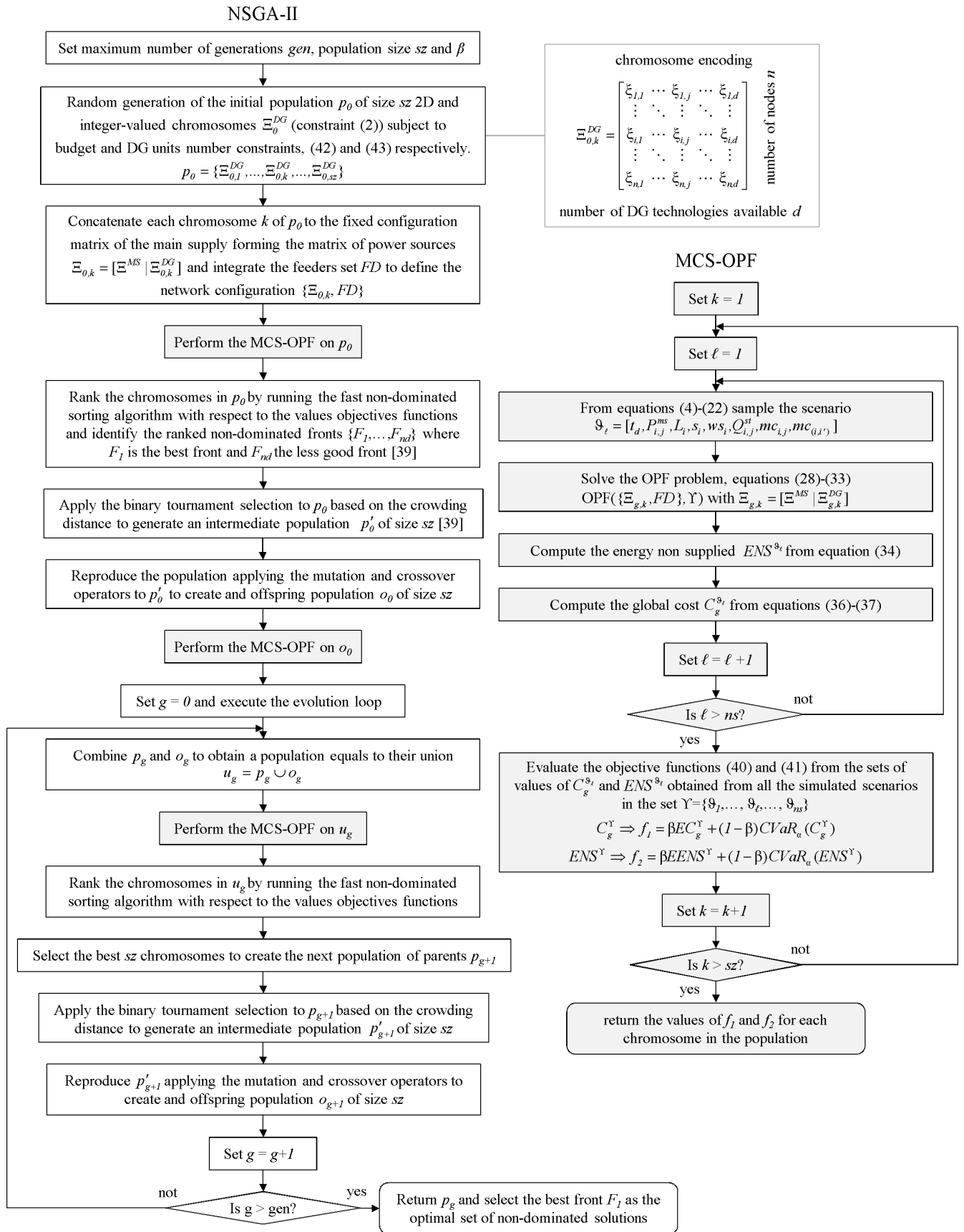
Figure 7. Flow chart of NSGA-II MCS-OPF MOO framework
