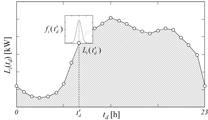
Figure 3. Daily load profile. Hourly normally distributed load
