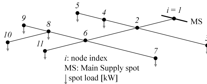
Figure 8. Radial 11-nodes distribution network
