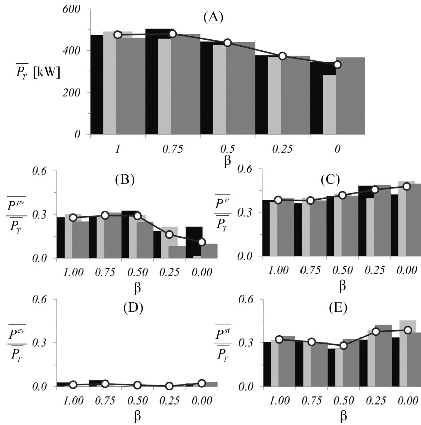
Figure 13. Average total DG power allocated (A) and its breakdown by type of DG: PV (B), W (C), EV (D) and ST (E)
