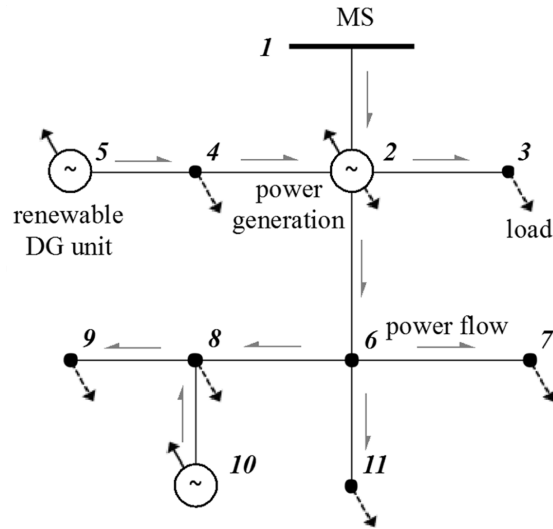
Figure 1. Example of distribution network configuration
