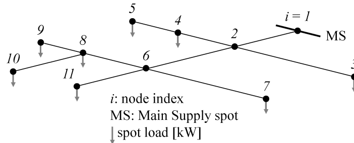
Figure 8. Radial 11-nodes distribution network
