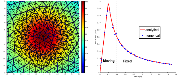
Fig. 4. Focus on the numerical V and E solutions on \Omega_M (left). Comparison between numerical and analytical solutions of E according to the radius (right).
