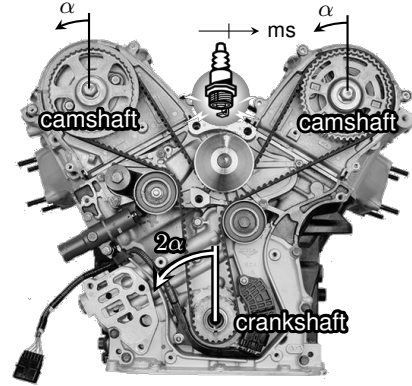
Fig. 5. Timing elements of a 4-stroke petrol engine
