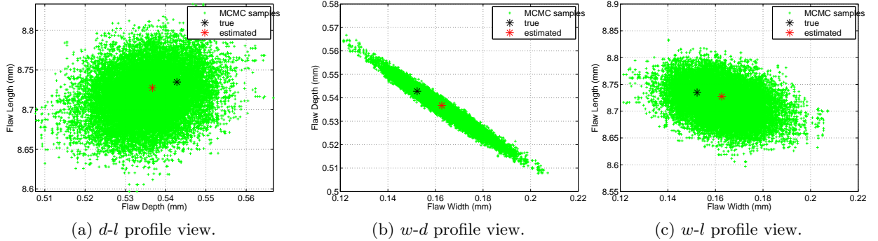
Figure 2: MCMC samples ( K = 10^5 , walk step t = [0.01, 0.01, 0.04] ) of random walk MWG method for tested sample d = 0.5428 mm, l = 8.7348 mm, w = 0.1523 mm. The estimated results are \hat{d} = 0.5385 \pm 0.0122 mm, \hat{l} = 8.7310 \pm 0.1739 mm and \hat{w} = 0.1597 \pm 0.0110 mm.
