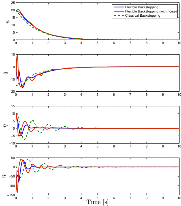
Fig. 4. Evolution of attitude, pitch rate and flexible states
