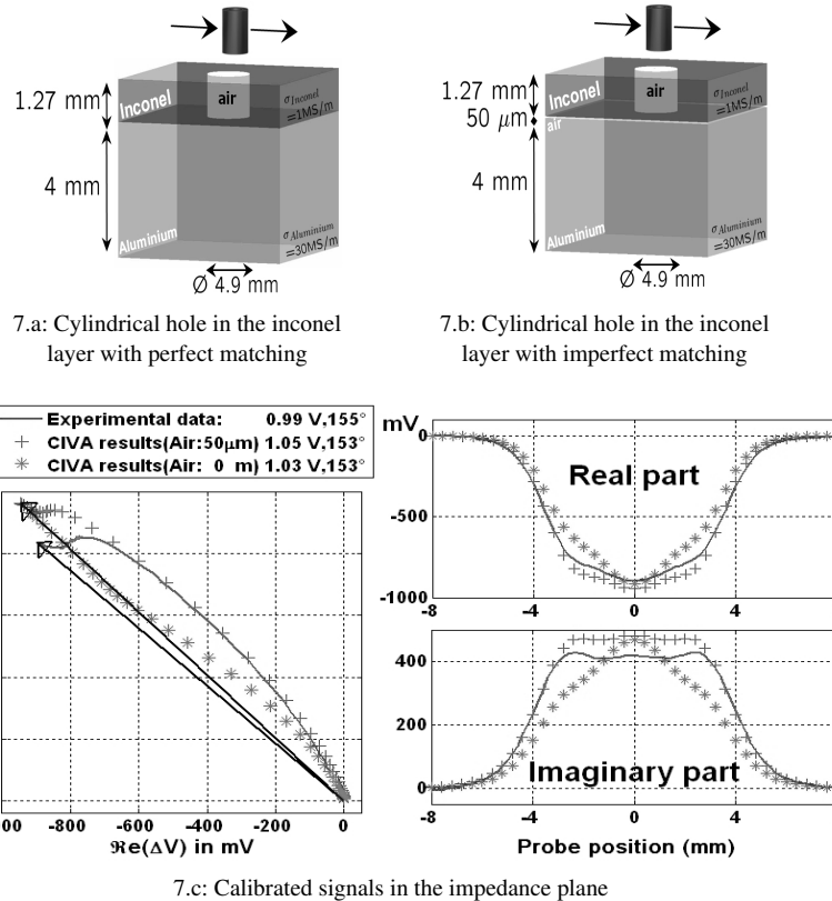
Figure 7. Cylindrical hole in the inconel layer of a two-layer slab perfectly matched (— experimental data, *** CIVA results with perfect matching, +++ CIVA results with imperfect matching)
