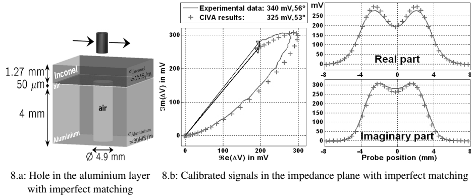
Figure 8. Cylindrical hole in the aluminium layer of a two-layer slab (— experimental data, +++ CIVA results)
