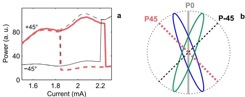
Figure 1. Experimental observations of the bistability. (a) Polarization LI curve at +45° (thick, red) and -45° (thin, black) for an increasing (solid) and a decreasing injection current (dashed). (b) Scheme of the different polarization states involved: linear polarization at threshold is the vertical gray line P0, and the two EP states around which the limit cycles oscillate are the two ellipses symmetrical with respect to P0. The dashed lines show the polarizations used for the measurement of the LI curve: +45° (thick red) and -45° (thin black).
