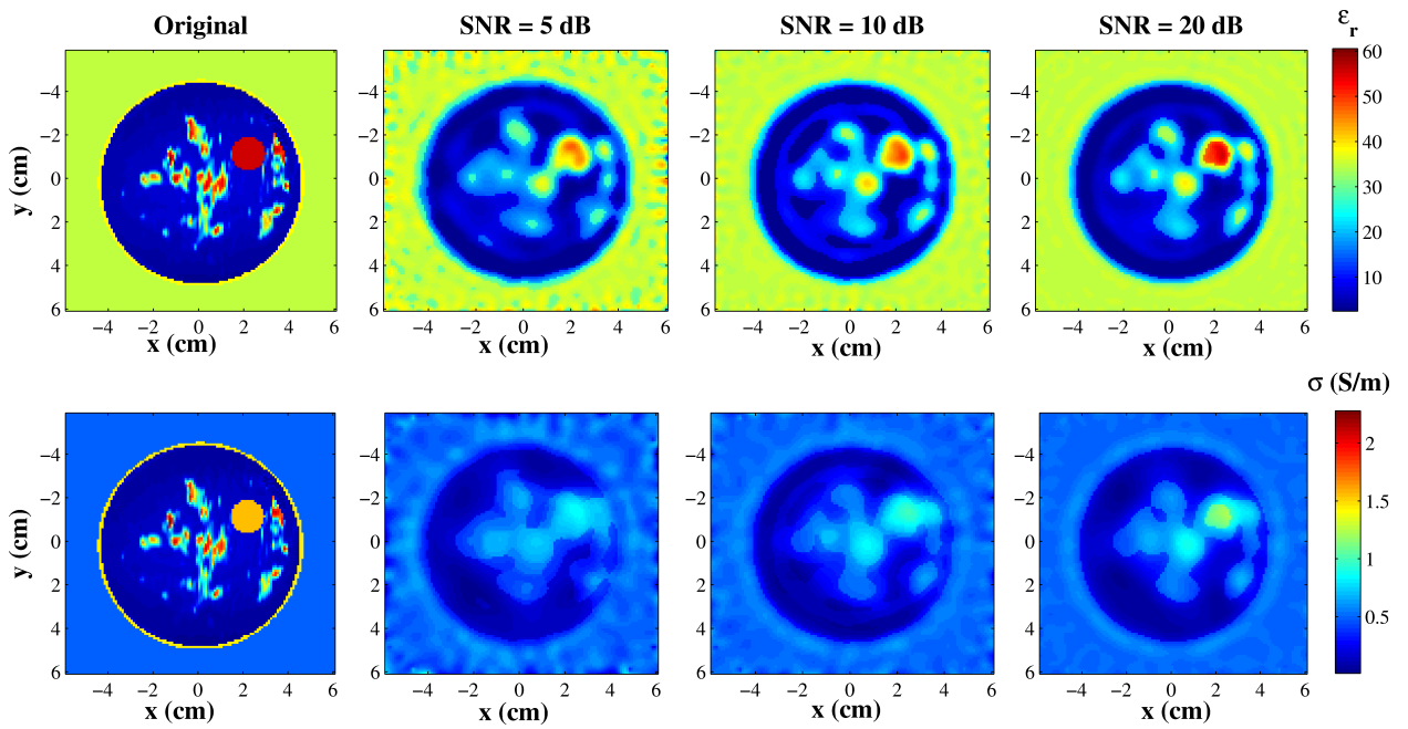
Fig. 8. Permittivity (top row) and conductivity (bottom row) maps of phantom 2 obtained from noisy data.
