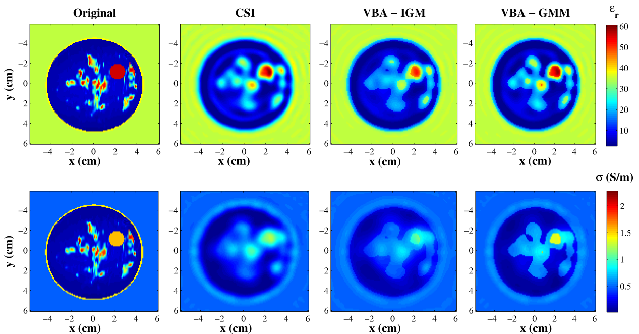
Fig. 5. Maps of permittivity (top row) and conductivity (bottom row) of phantom 2 reconstructed by means of CSI (2nd column) and VBA with the IGM (3rd column) and GMM (4th column) a priori models compared with the actual object (1st column).
