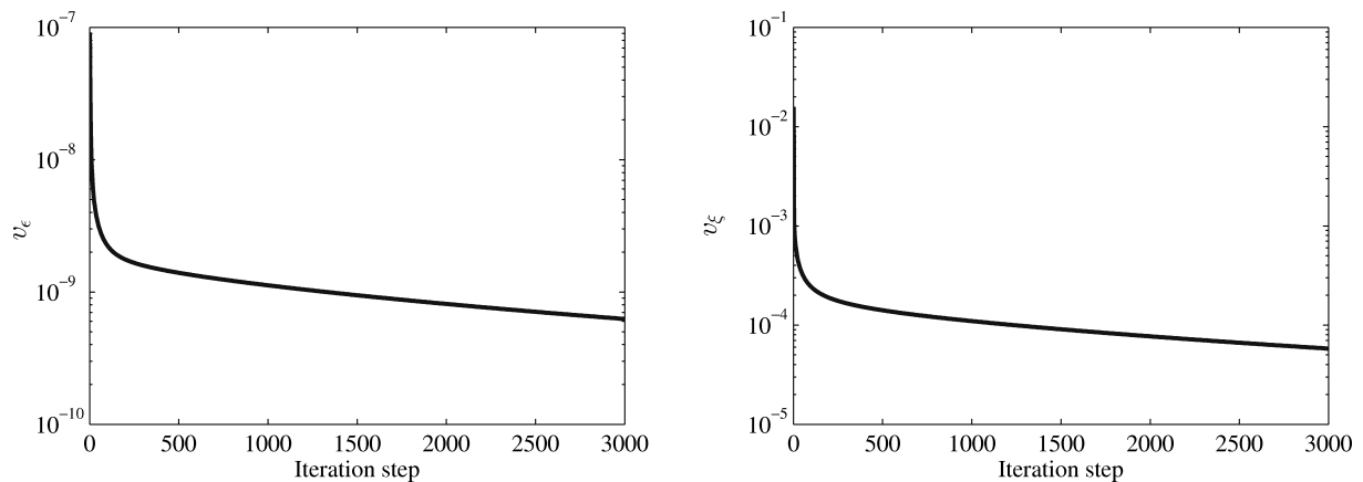
Fig. 3. The evolution of the observation v_\epsilon (left) and coupling v_\xi (right) error variances as functions of the iteration step for phantom 1.
