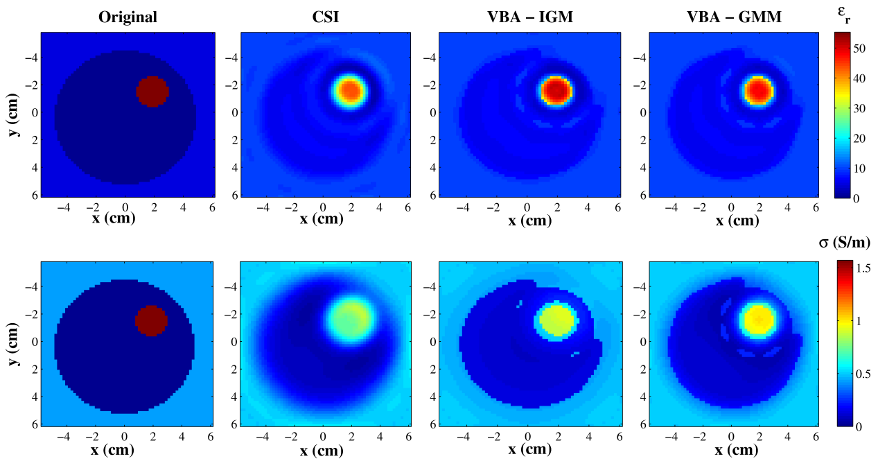
Fig. 4. Maps of permittivity (top row) and conductivity (bottom row) of phantom 1 reconstructed by means of CSI (2nd column) and VBA with the IGM (3rd column) and GMM (4th column) a priori models compared with the actual object (1st column).
