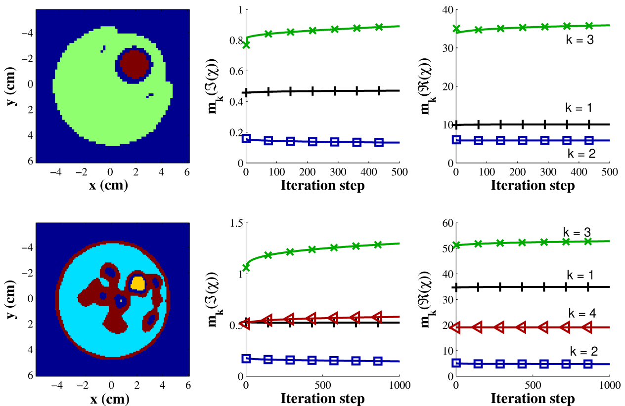
Fig. 6. Hidden fields (left) and means m_k of the real (right) and imaginary (middle) parts of the contrast corresponding to different classes for phantoms 1 (top row) and 2 (bottom row).
