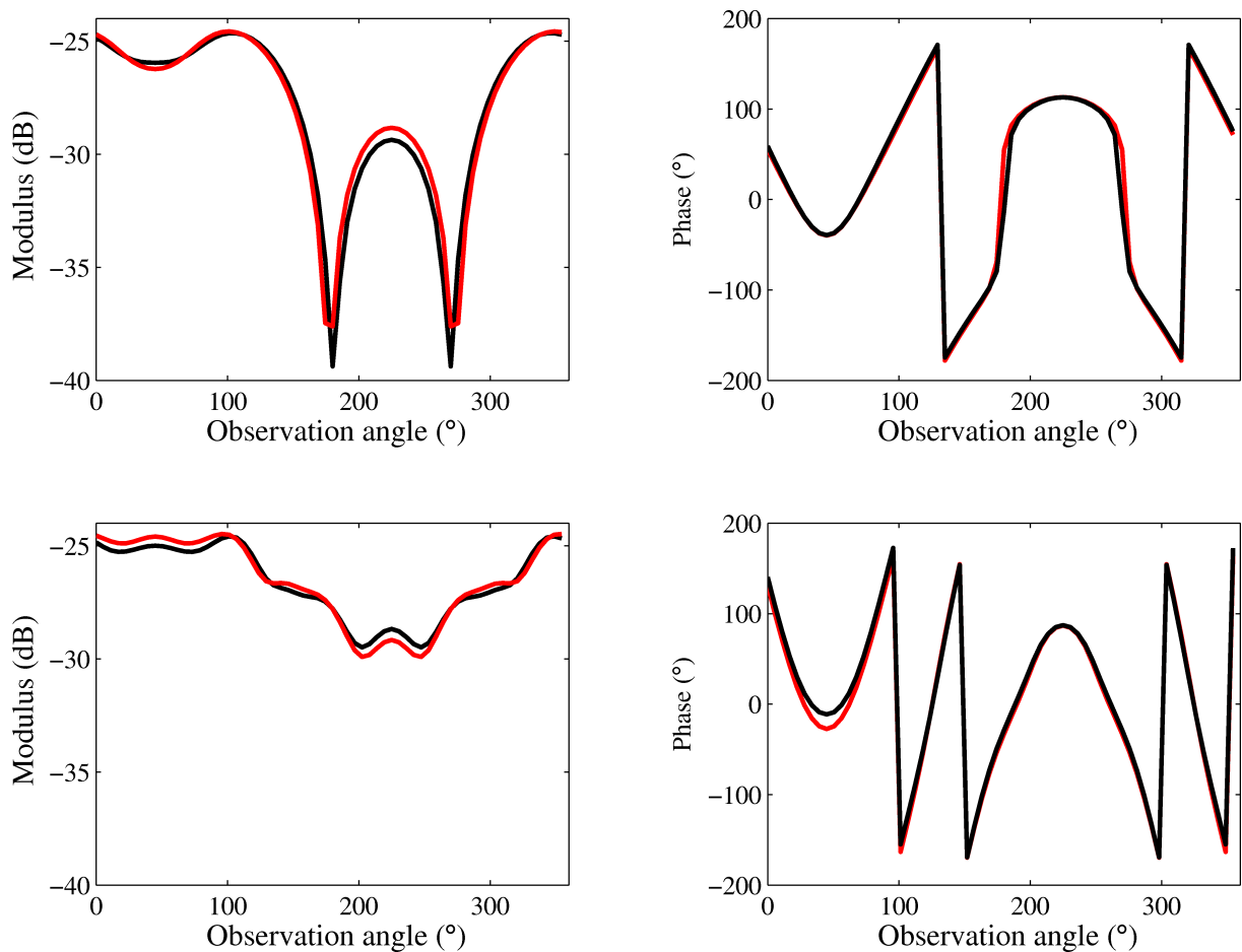
Fig. 2. Amplitude (left) and phase (right) of the scattered fields computed by means of the data model (black line) and by means of the forward model used for inversion (red line) at 1.5 GHz (top) and 3 GHz (bottom).
