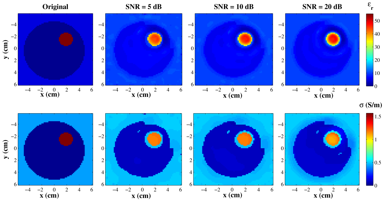
Fig. 7. Permittivity (top row) and conductivity (bottom row) maps of phantom 1 obtained from noisy data.
