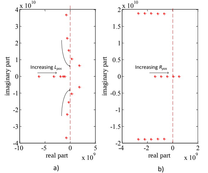
Fig. 3. Root locus a) R_{pos} = 0 and increasing values of L_{pos} b) L_{pos} = 5 nH and increasing values of R_{pos}
