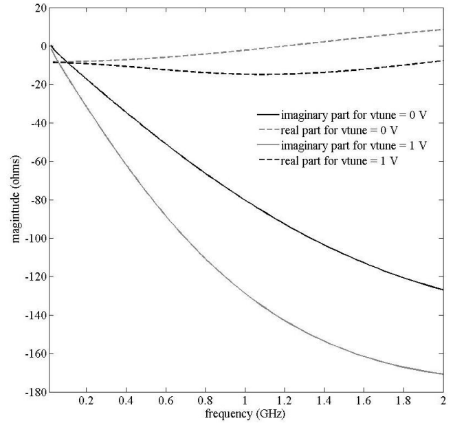
Fig. 6. Imaginary and real part of the input impedance of the IC layout for different values of V_{tune}
