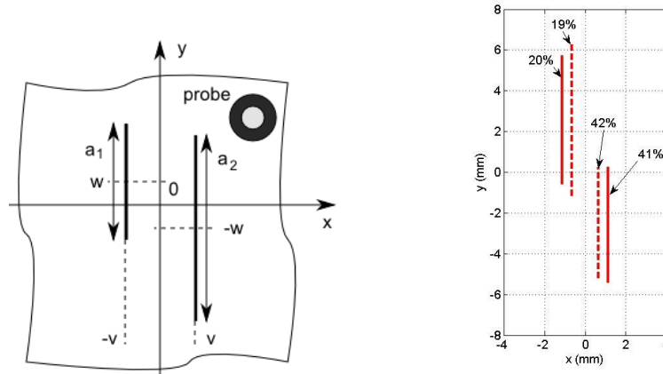
Fig. 1 Left : top view of the plate with the two parameterized cracks and the scanning probe. Right : reconstruction results in a test case. Solid/dashed lines: real/found cracks. Depths are shown in percentage of the plate thickness.
