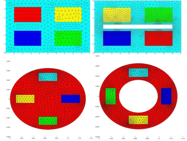
Figure 1: Non-collocated piezoelectric patches bonded on structures.
