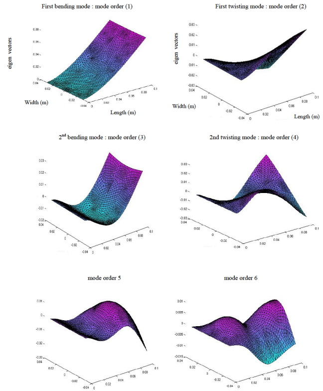
Figure 5: Modes shapes of the system
