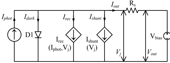
Fig. 6. Schematic of the electrical model of a a -Si cell, consisting of a current source, a diode, a series resistance, a recombination current term (as described by Merten et al. [38]), and a shunt current term (as described by Bishop [36]).
