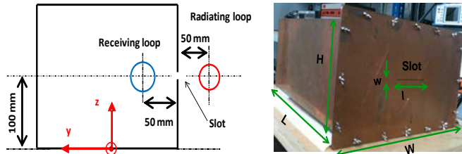
Fig. 7. Modeled structure
