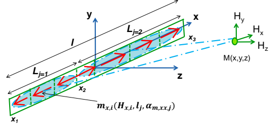
Fig. 3. Magnetic moment dipole distribution in slot (case 2).
