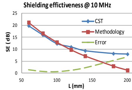
Fig. 9. Limit of methodology at 10 MHz
