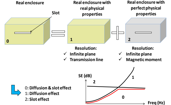
Fig. 6. Shielding of enclosures using proposed methodology
