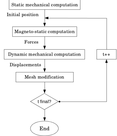
Fig. 5. Simulation algorithm
