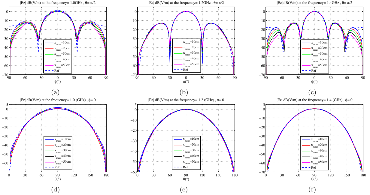
Figure 11: Comparison of the FF radiation pattern for x_{meas} = 10cm, 20cm, 30cm, 40cm and 50cm at the plane cut \theta = \pi/2 , (a) at 1GHz , (b) at 1.2GHz , (c) at 1.4GHz . Comparison of the FF radiation pattern at the plane cut \phi = 0 , (d) at 1GHz , (e) at 1.2GHz , (f) at 1.4GHz .
