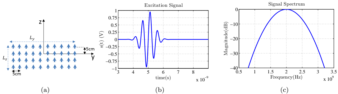
Figure 1: The time-domain excitation signal (b) applied to each of the 40 dipoles composing the AUT (a) and the magnitude of the excitation signal spectrum (c). The maximum of the spectrum is at 2\text{GHz} .
