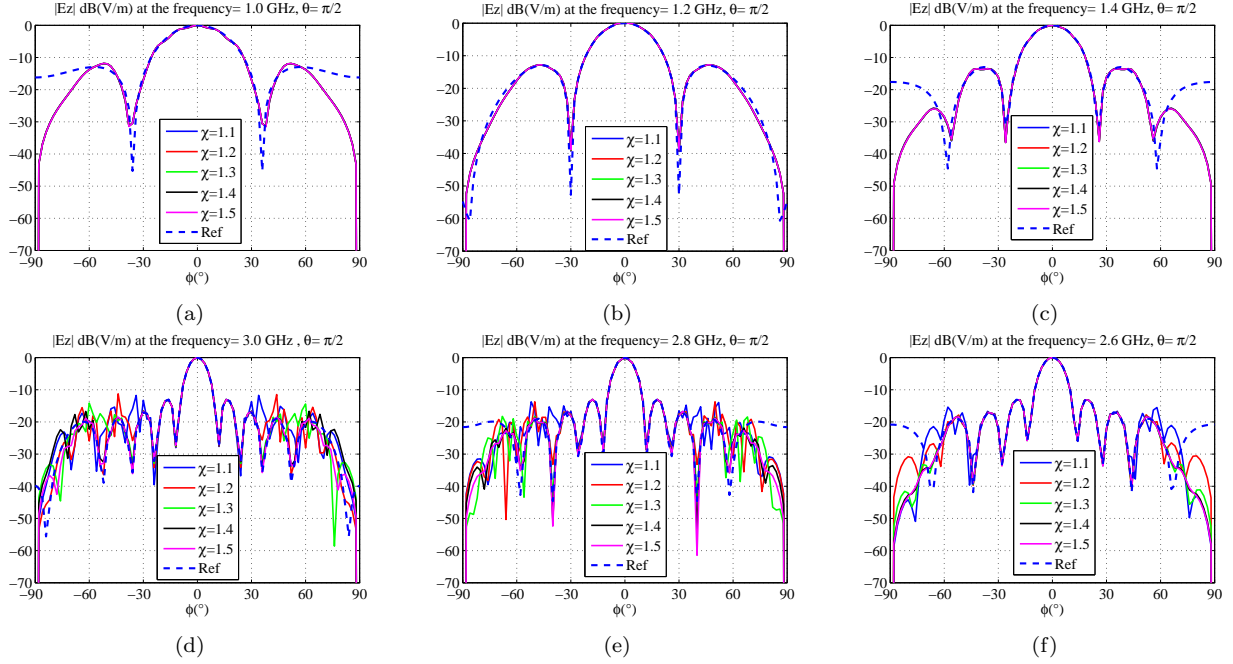
Figure 8: Comparison of far-field E_z -component at the plane cut \theta = \pi/2 with D_{max} = 150cm , x_{meas} = 50cm and \Delta y = \Delta z = \lambda_0/2\chi for \chi = 1.1, 1.2, 1.3, 1.4, 1.5 . (a-d) For 1GHz and 3GHz ( F_{-30dB} ) respectively. (b-e) For 1.2GHz and 2.8GHz ( F_{-20dB} ) respectively. (c-f) For 1.4GHz and 2.6GHz ( F_{-10dB} ) respectively.
