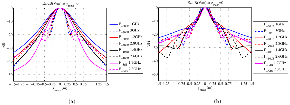
Figure 9: The normalized E_z NF component for F_{-30dB} ( 3GHz, 1GHz ), F_{-20dB} ( 2.8GHz, 1.2GHz ), F_{-10dB} ( 2.6GHz, 1.4GHz ), F_{-3dB} ( 2.3GHz, 1.7GHz ). (a) At the plane cut y_{meas} = 0 . (b) At the plane cut z_{meas} = 0 .
