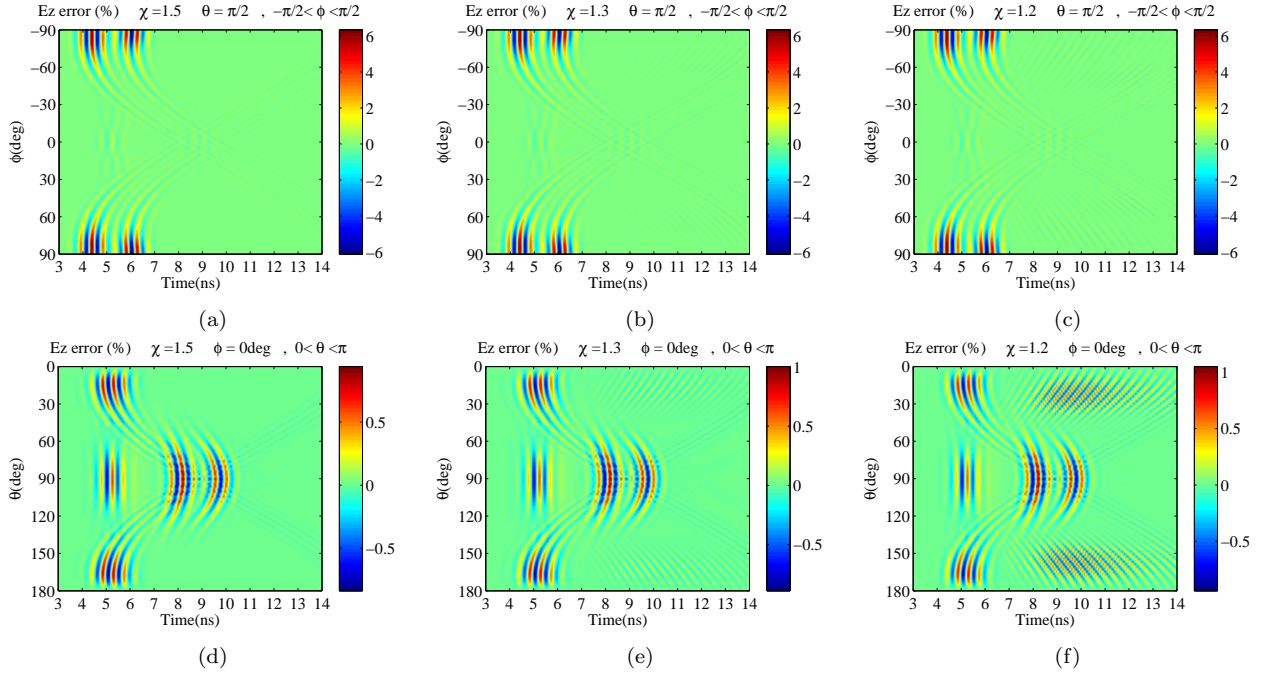
Figure 6: The FF Ez component error as a function of time for the plane cut \theta = \pi/2 . (a) for \chi = 1.5 , (b) for \chi = 1.3 , (c) for \chi = 1.2 . The Ez error as a function of time for the plane cut \phi = 0 , (d) for \chi = 1.5 , (e) for \chi = 1.3 , (f) for \chi = 1.2 .
