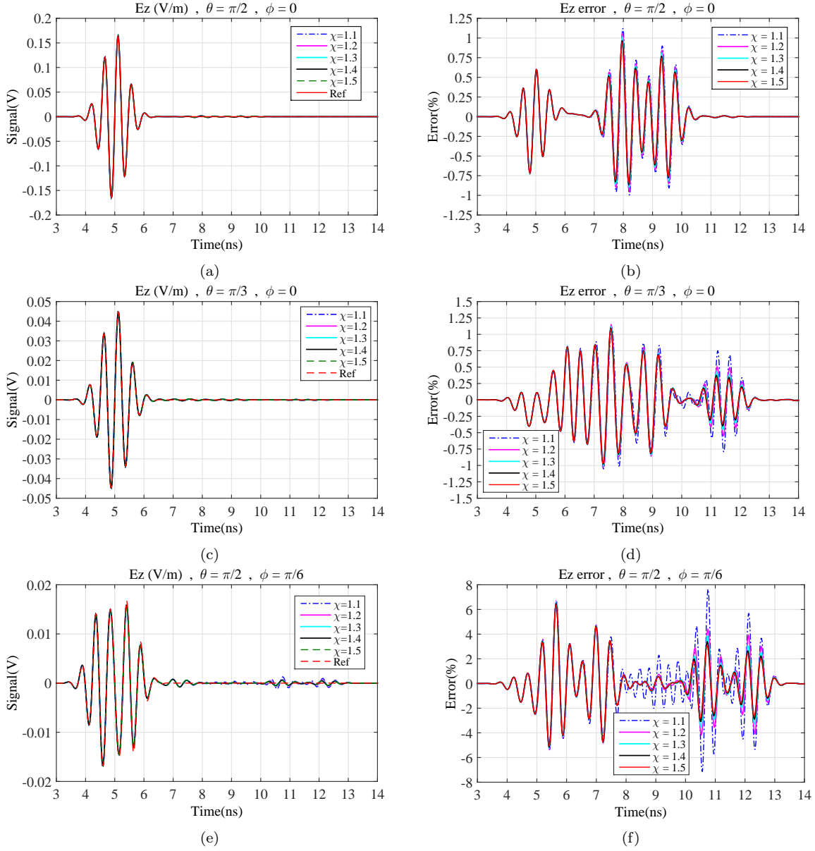
Figure 5: Comparison of the NF to FF transformation results for different sampling criteria \Delta y = \Delta z = \lambda_0/2\chi , D_{max} = 150cm and x_{meas} = 50cm . The TD FF E_z component at (a) \theta = \pi/2 and \phi = 0 , (c) \theta = \pi/3 and \phi = 0 (e) \theta = \pi/2 and \phi = \pi/6 . The errors of Figs. (a-c-e) are respectively (b) \theta = \pi/2 and \phi = 0 , (d) \theta = \pi/3 and \phi = 0 (f) \theta = \pi/2 and \phi = \pi/6 .
