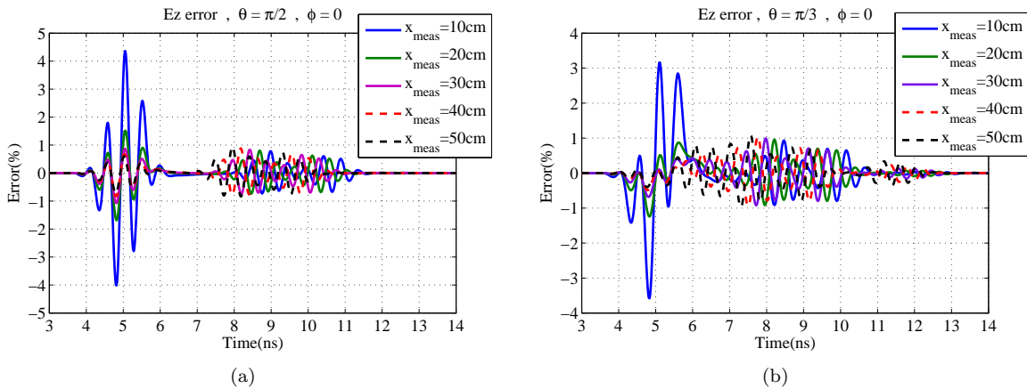
Figure 10: The Ez error as a function of time and as a function of the NF measurement distance ( x_{meas} ) for the FF observation points (a) \theta = \pi/2 and \phi = 0 , (b) \theta = \pi/3 and \phi = 0 .
