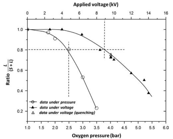
Fig. 3. Evolution of the melting zone, through the ratio L/(S+L) , as a function of the applied voltage and oxygen pressure ( \text{BaCo}_2\text{V}_2\text{O}_8 ). Liquid ( L ) and solid ( S ) parts were determined by analyzing the camera pictures of the melting zone (see Fig. 2).
