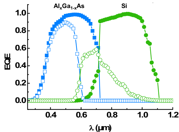
Fig. 3. External Quantum Efficiency (EQE) versus photon wavelength of two current matched \text{AlGaAs}/\text{Si} tandem cells. The blue square and green circle symbols represent the individual EQE of the top and the bottom cells respectively. J_{sc} \sim 19\text{mA}/\text{cm}^2 is obtained for a 1.16\mu\text{m} \text{Al}_x\text{Ga}_{1-x}\text{As} top cell with x=0.24 and for a 500\mu\text{m} Si bottom cell (full symbols). J_{sc} \sim 9\text{mA}/\text{cm}^2 is obtained for a 1.24\mu\text{m} \text{Al}_x\text{Ga}_{1-x}\text{As} top cell with x=0.56 and for a 5\mu\text{m} Si bottom cell (open symbols).
