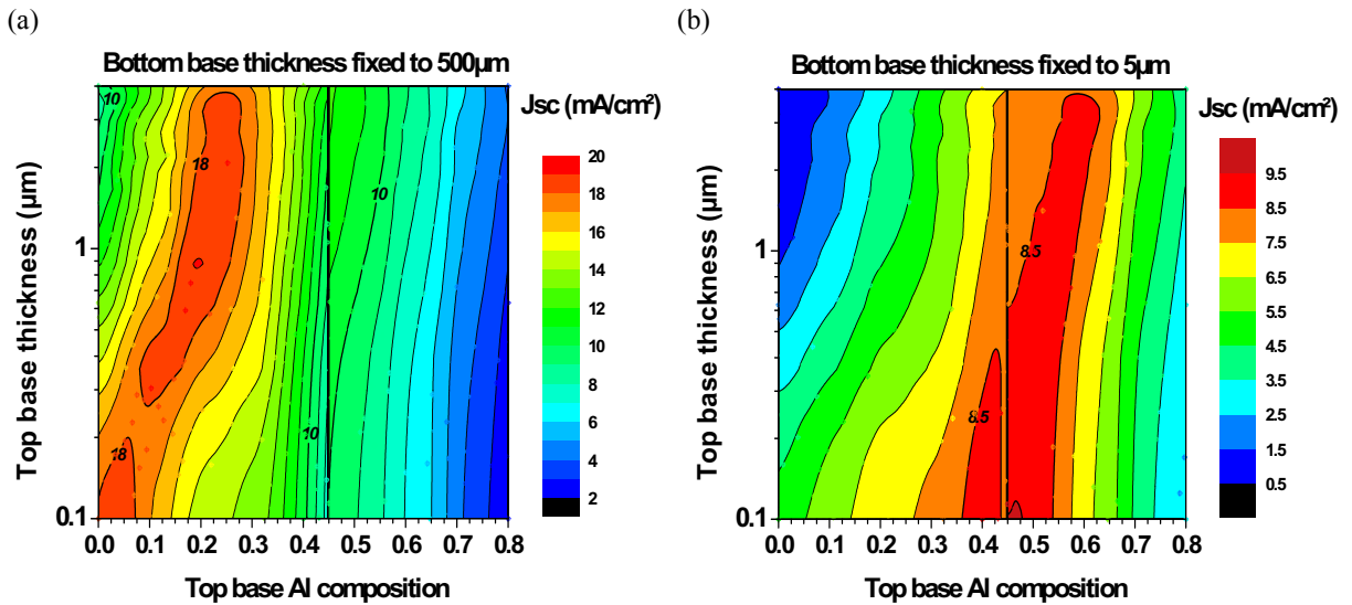
Fig. 2. Maps of tandem cell short circuit densities ( J_{sc} ) simulated for different combinations of Aluminum compositions and thicknesses of the top base: (a) for a thick Si bottom cell ( 500\mu m ) and (b) for a thin Si bottom cell ( 5\mu m ). The solid lines for x=0.45 represent the border between direct and indirect band gap for AlGaAs .
