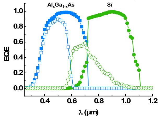
Fig. 3. External Quantum Efficiency (EQE) versus photon wavelength of two current matched AlGaAs/Si tandem cells. The blue square and green circle symbols represent the individual EQE of the top and the bottom cells respectively. J_{sc} \sim 19 mA/cm^2 is obtained for a 1.16\mu m Al_xGa_{1-x}As top cell with x=0.24 and for a 500\mu m Si bottom cell (full symbols). J_{sc} \sim 9 mA/cm^2 is obtained for a 1.24\mu m Al_xGa_{1-x}As top cell with x=0.56 and for a 5\mu m Si bottom cell (open symbols).
