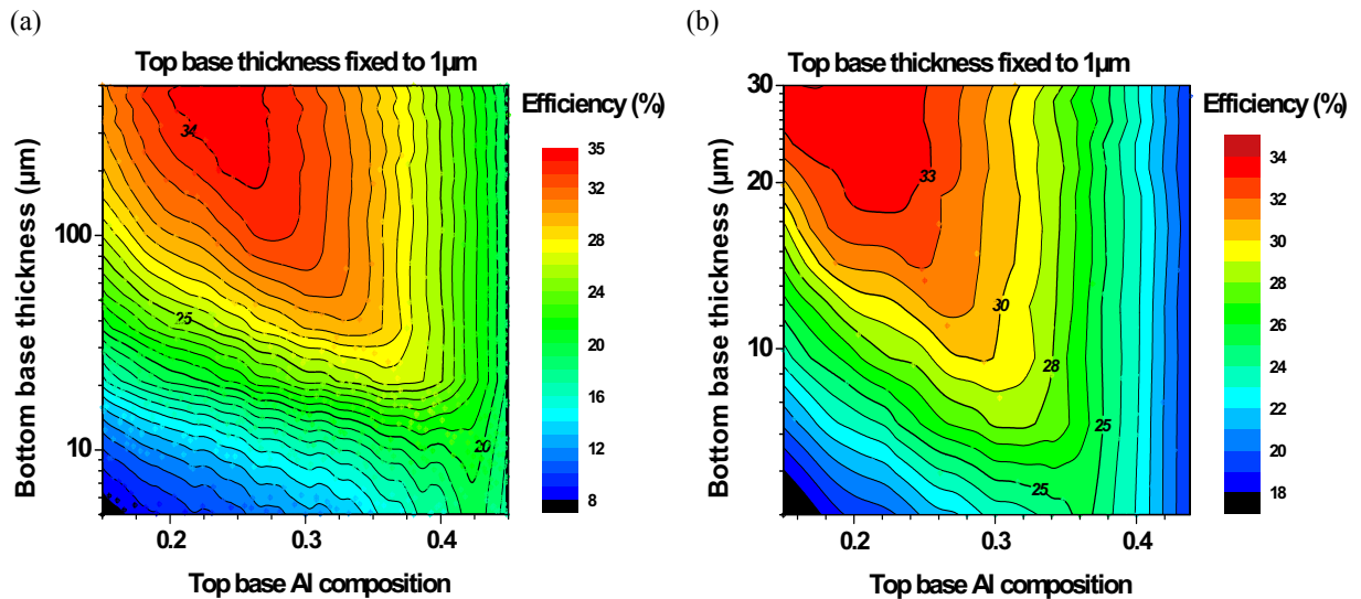
Fig. 4. Maps of tandem cell efficiencies simulated for different combinations of top base Aluminum compositions and bottom base thicknesses: (a) for a bottom cell in epi-Si and (b) for a bottom cell in epi- \text{Si}_{0.63}\text{Ge}_{0.27} .
