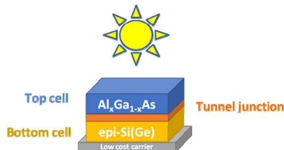
Fig. 1. Simplified schematic of the novel concept of the AlGaAs/epi-Si(Ge) tandem solar cells. More detailed information on each layer can be found in Table 1.
