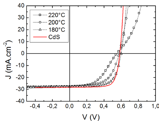
FIG. 10. J-V characteristics of solar cells with buffers of indium content \text{In}/(\text{In} + \text{Zn}) close to 28 at. % as a function of the buffer layer deposition temperatures. Illumination AM1.5 100 \text{ mW}\cdot\text{cm}^{-2} .
