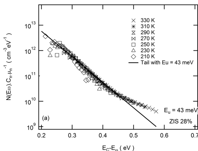
FIG. 4. Example of MPC density of states spectra for sample with ZIS of 28%.
